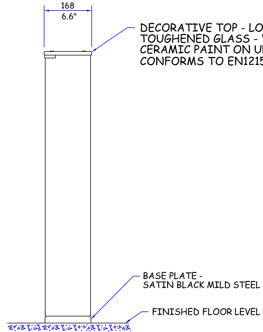
END VIEW
